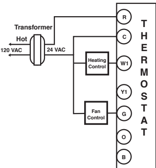
HEAT ONLY 3-WIRE SINGLE TRANSFORMER
