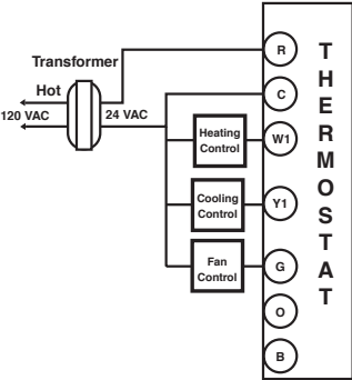
HEAT/COOL 4-WIRE SINGLE TRANSFORMER
