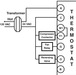
HEAT PUMP WITH COOL ACTIVE REVERSING VALVE
