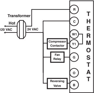
HEAT PUMP WITH HEAT ACTIVE REVERSING VALVE
