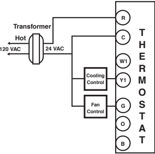
COOL ONLY 3-WIRE SINGLE TRANSFORMER
